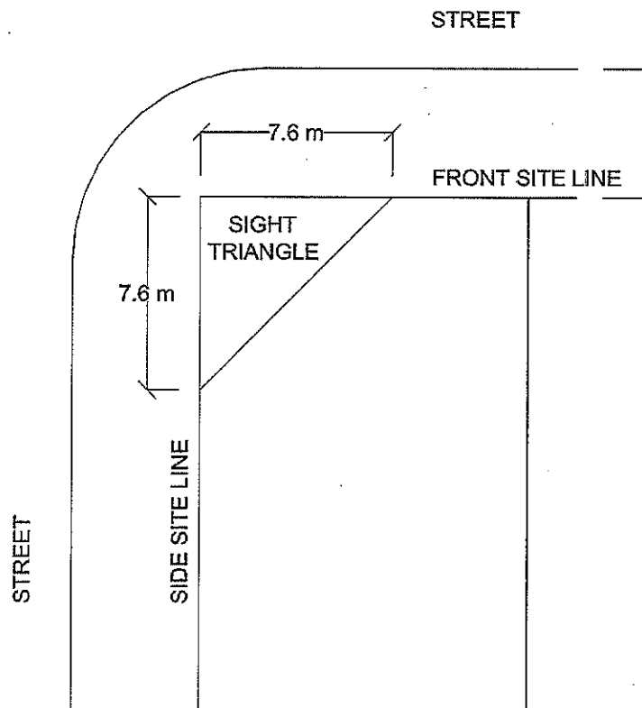
Figure 2-2: Sight Triangle
