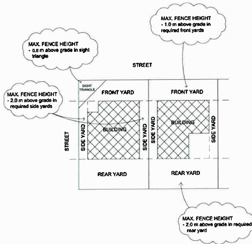
Figure 4-1: Fence Requirements
