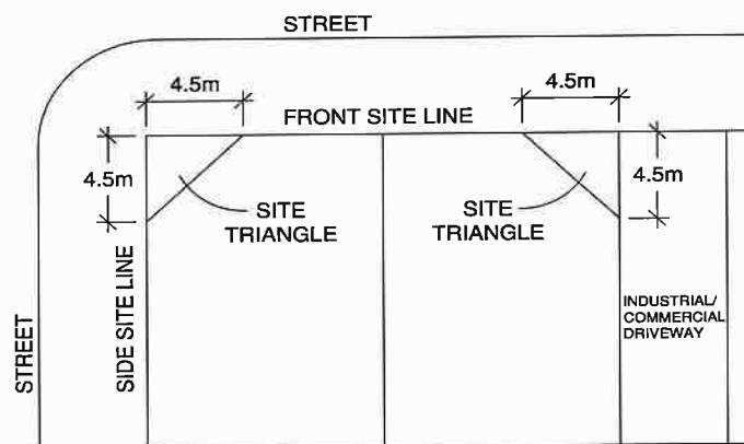
Figure 2-1: Sight Triangles
